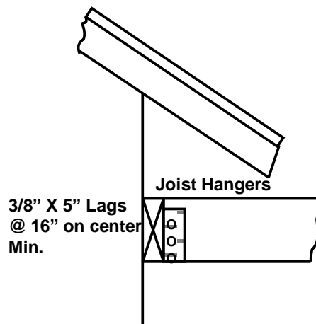
LEDGER DETAIL
