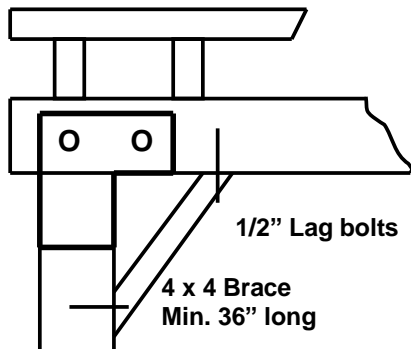
KNEE BRACE DETAIL
