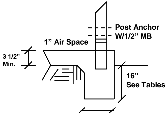
FOOTING DETAIL
