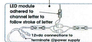
LED Channel letter installation example
