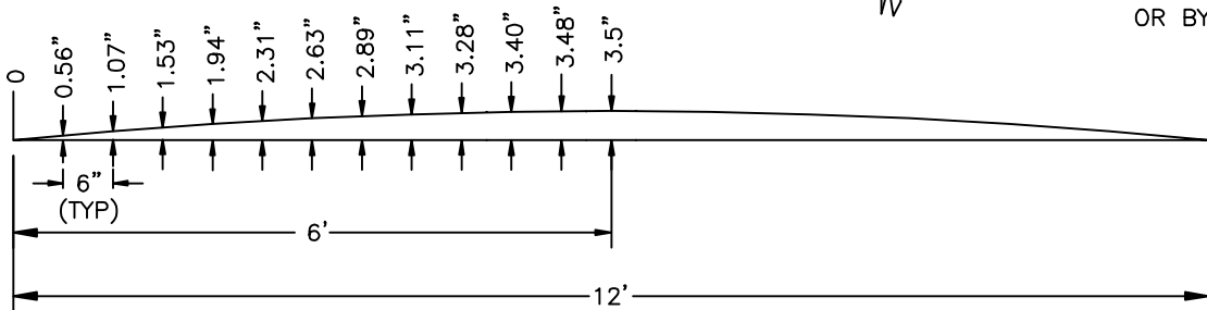
SECTION B-B
