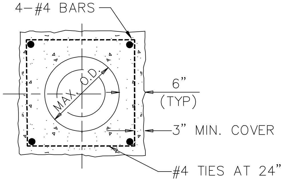
CROSS SECTION OF ENCASEMENT
